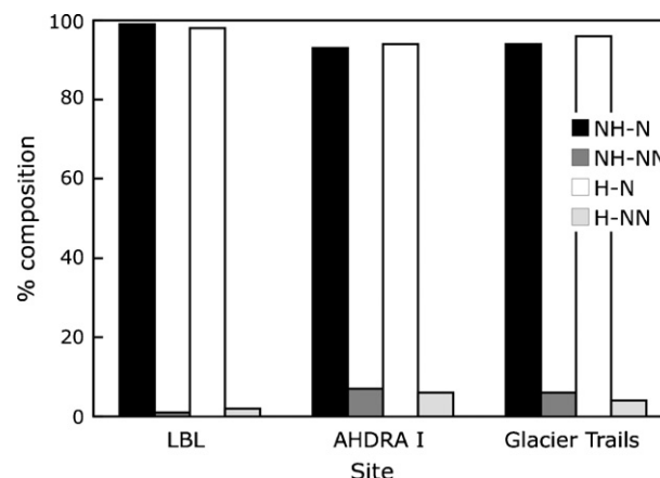
Fig. 3. Comparison of the percent composition of native (N) and non-native (NN) plant species observed for the five transects perpendicular to trails where horses are prohibited (NH = no horse) and allowed (H = horses allowed). All values are based on the average of all plots along the 50 m transect that was perpendicular to the trail.
